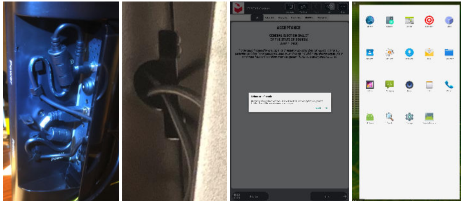
Figure 13: Rebooting the ICX into Safe Mode. Left to right: (1) The ICX power button is located behind a plastic door on the side of the machine; (2) Even with the door closed, an opening for cables allows the button to be pressed by inserting a metal tool; (3) Holding the button causes the machine to show a “Reboot to safe mode” prompt; (4) When the machine reboots, the user has unrestricted access to Android, including the ability to install malware.
